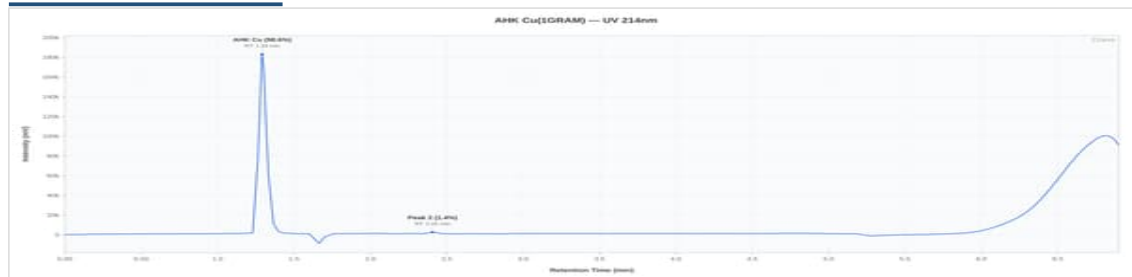
AHKCU RAW 1GRAM - AHK1G26N: UV Chromatogram
