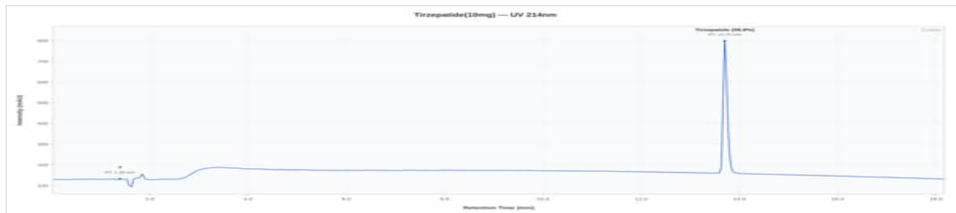
Adamax 10mg - NLL-2825133: UV Chromatogram
