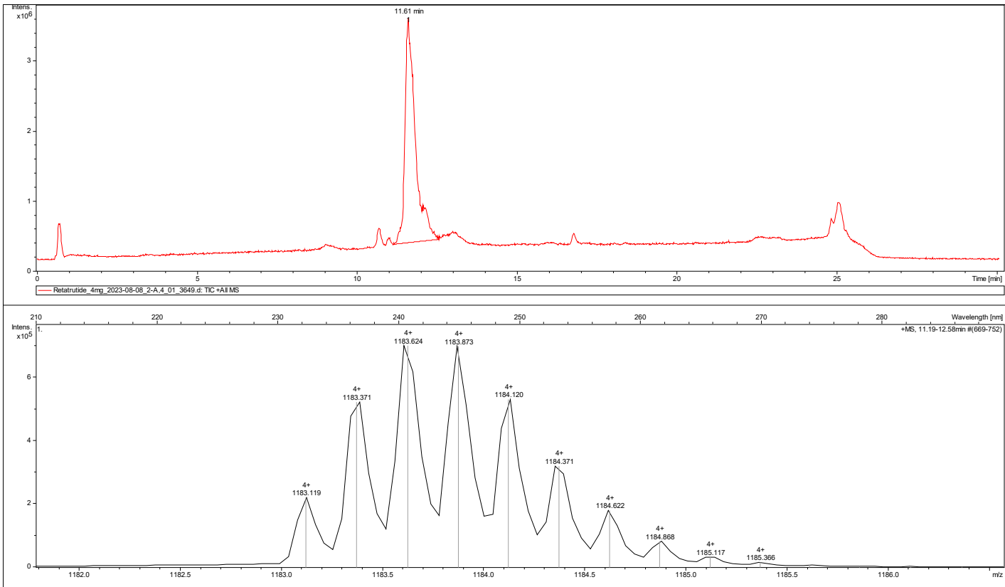
Top panel, LC-MS total ion current Bottom panel, positive scan Zoomed to base peak 1183.6 Da
