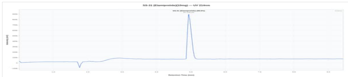
SS31 10mg - NLL-4091611: UV Chromatogram
