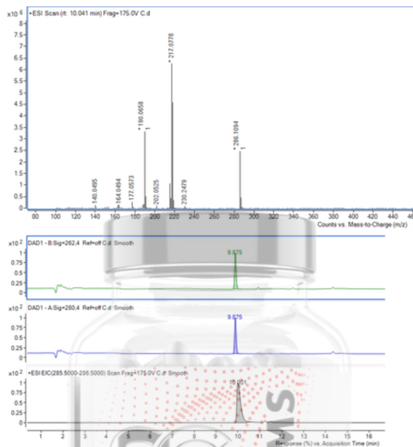
Fig.1 MS pectrum of Letrozole in positive mode; LC-UV graph and ESI-EIC graph of Letrozole
